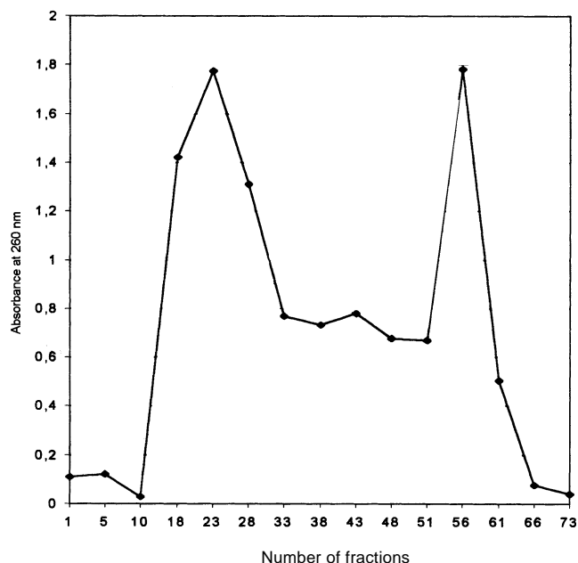
Figure 3. Results of elution of extract from yeast biomass growth in static conditions through Sephadex G-75 column.
