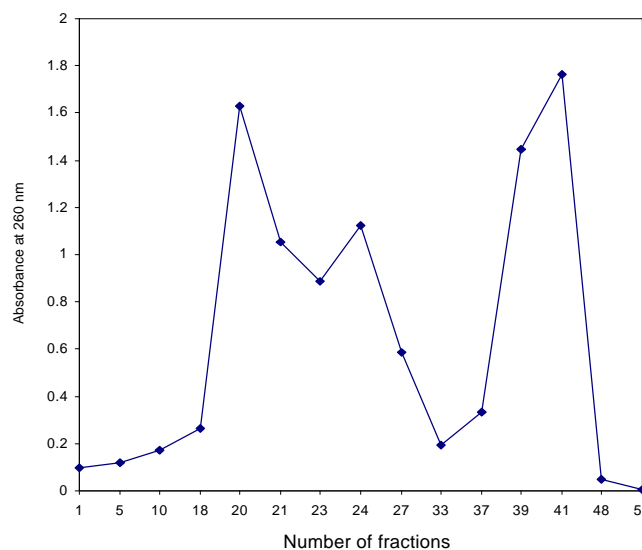
Figure 4. Results of elution of extract from yeast biomass growth in semiaerobic conditions through Sephadex G-75 column.
