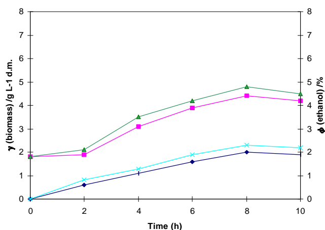
Figure 1. Dynamics of biomass and ethanol production in static conditions with 200 mg/l of CrCl 3 and without addition of CrCl 3 into the molasses medium. (■, ▲), Biomass (medium without '■' and with '▲' addition of chromic chloride). (●, ×) Ethanol (medium without '●' and with '×' addition of chromic chloride).
