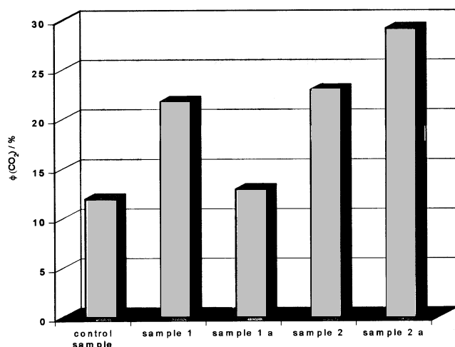
Figure 5. Stimulation of CO 2 production by addition of GTF into the synthetic medium from samples 1, 1a, 2 and 2a. Samples 1 and 1a: GTF in fraction No. 18–51 (sample 1) and No. 52–61 (sample 1a) from yeast biomass extract. Cells growth in static conditions. Samples 2 and 2a: GTF in fraction No. 19–22 (sample 2) and No. 23–27 (sample 2a) from yeast biomass extract. Cells growth in semiaerobic conditions.
