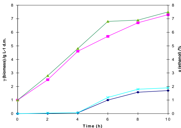
Figure 2. Dynamics of biomass and ethanol production in semiaerobic conditions with 200 mg/l of \text{CrCl}_3 and without addition of \text{CrCl}_3 into the molasses medium. (■, ▲), Biomass (medium without '■' and with '▲' addition of chromic chloride). (●, ×) Ethanol (medium without '●' and with '×' addition of chromic chloride).
