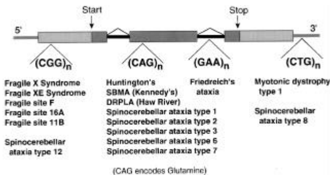
Figure 1. Location of repeat tract in triplet repeat diseases genes. An idealized gene is shown with the dark shaded area representing the coding region. The transcription start and stop are indicated. The light shaded area represents the 5' upstream and 3' downstream untranslated regions (UTR). Introns are shown as black lines and the flanking region as a shaded line. Both disease-associated (CGG)_n triplet repeats and three fragile sites are located in the 5' UTR. The (CAG)_n repeat in SCA-12 is also located in the 5' UTR. Many glutamine encoding CAG repeats are located within exons of the gene coding regions. The (GAA)_n repeat in Friedreich's ataxia is located in an intron. The (CTG)_n repeats in myotonic dystrophy type 1 and SCA-8 are located in the 3' UTR of associated genes.
