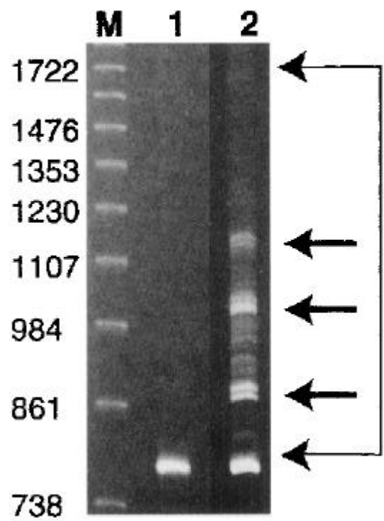
Figure 3. Slipped strand DNA structures migrate as heterogeneous products with reduced mobility on polyacrylamide gels. Lane 1, ladder of molecular weight markers. Lane 2, 878 bp DNA fragment containing (CTG)_{255} \cdot (CAG)_{255} (with several sequence interruptions) derived from the DM locus. Following denaturation and renaturation many slow migrating bands (bracketed area), including three major pairs of doublets (arrows) are observed.
