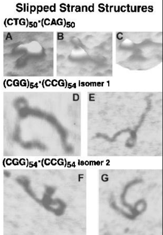
Figure 10. AFM images of representative slipped strand DNA structures. AFM images A–C show three-dimensional projections of three slipped strand DNA molecules [the most slowly migrating product as described (Pearson et al 1998b)] from (CTG) 50 •(CAG) 50 . A pyramidal structure is observed at the apex of a bent molecule. One interpretation is that this pyramidal mass represents two looped out strands interacting above the plane of the DNA molecule. AFM images D–E and F–G are the two major slipped strand isomers from (CGG) 54 •(CCG) 54 . A clear loop is seen in AFM images from both of these structural isomers. Again this may be the interaction of two long loop out structures or the looping of the very flexible (CGG)•(CCG) linear helix held together by interactions between short loops.
