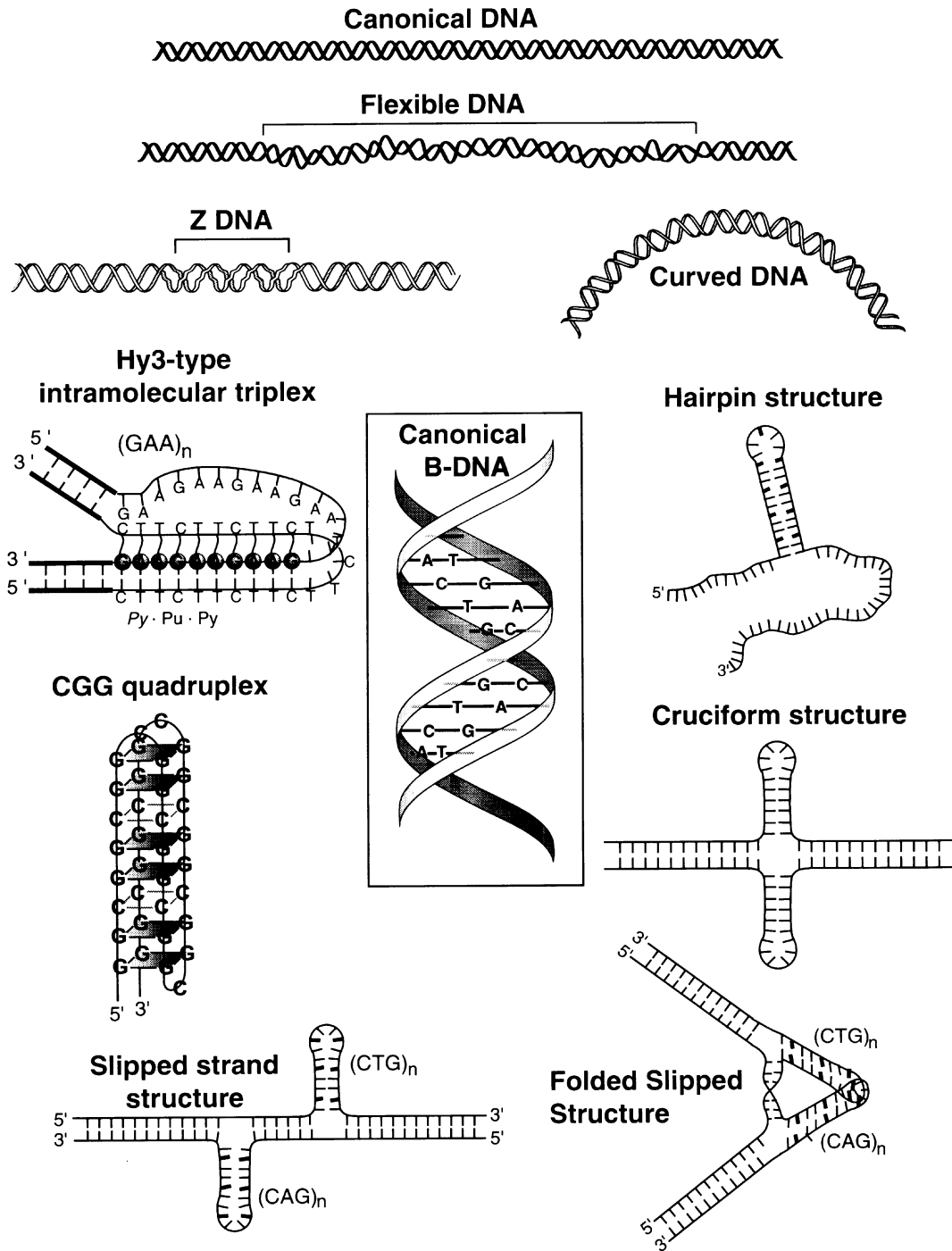
Figure 2. Alternative DNA structures formed in repeated DNAs. A canonical B-form helix is shown in a box in the center of the figure. A representation of this helix is also shown at the top of the figure. Although a straight molecule is shown, the DNA inherently possesses a certain degree of flexibility. (CTG)_n \bullet (CAG)_n and (CGG)_n \bullet (CCG)_n repeats, however, are extremely flexible compared to mixed sequence B-form DNA (shown below canonical DNA). The next two representations, Z-DNA and stable curved DNA, occur in (CG)_n \bullet (CG)_n and (GT)_n \bullet (AC)_n runs and DNA containing phased A_{4-5} \bullet T_{4-5} tracts (and other sequences), respectively, but have not been identified in triplet repeats. Proceeding clockwise, hairpin structures form in most disease-relevant triplet repeat single strands (to some degree). Cruciform structures form in perfect inverted repeats and have not been identified in triplet repeat sequences. Folded slipped strand structures and simple slipped strand structures form in (CTG)_n \bullet (CAG)_n and (CGG)_n \bullet (CCG)_n repeats, as discussed in the text. Quadruplex structures have been identified in oligonucleotides containing CGG and TGG repeats. In these structures the guanines are held together by G•G Hoogsteen bonds. A Hy3-type intramolecular triplex (as well as bi-triplex structures) can form in the (GAA)_n \bullet (TTC)_n repeat associated with Friedreich's ataxia.
