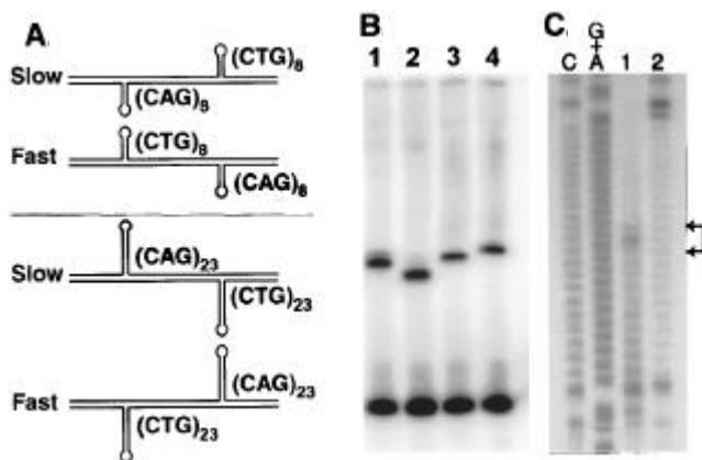
Figure 9. Properties of model slipped DNA constructs: effects of potential loop-loop interactions. (A) Different migration orders for heteroduplex isomers with short (non-interacting) and long (possibly interacting) triplet repeat loops. (B) The migration order for the long loops when the random sequences in two DNA strands cannot interact due to non-complementarity (lanes 1, 2) and when they are complementary (lanes 3, 4). Both pairs show 3' and 5' loop-outs in the top strand, respectively, as for the top pair of structures in A. (C) Chloroacetaldehyde reactivity of unpaired adenines and cytosines when the heteroduplex contains a single (CAG)_{23} loop (lane 1), and when it contains a complementary (CTG)_{23} loop 30 bp apart making an inter-loop interaction possible (lane 2).
