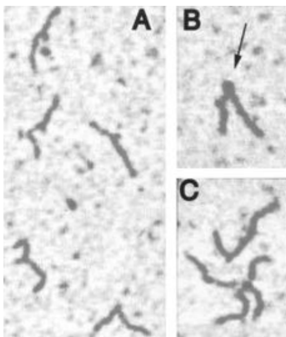
Figure 8. AFM images of (CTG)_{23} and (CAG)_{23} loop-outs. (A) Molecules with a single (CTG)_{23} loop-out. (B) A molecule with both a (CTG)_{23} and (CAG)_{23} loop-out in opposite strands with 30 bp spacing. The two complementary loop-outs likely interact forming a bulky protrusion indicated by the arrow. (C) Representative dimer molecule, where interactions of complementary loops of the two double loop-out fragments stabilize the association of two molecules.
