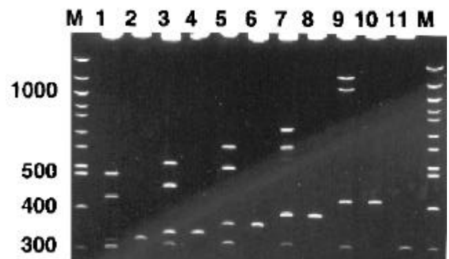
Figure 5. Electrophoretic separation in a polyacrylamide gel of 3-way junction heteroduplex isomers containing hairpins. This gel shows the separation of the hybridization products in a 5% native polyacrylamide gel. PvuII -digested plasmids with inserts in the EcoRI site were hybridized with PvuII -cut pUC8 and the products were separated in a polyacrylamide gel. The hybridization products contain 7 bp (lane 1), 12 bp (lane 3), 18 bp (lanes 5, 12), 27 bp (lane 7), and 50 bp (lane 9) hairpins. PvuII -digested insert-containing plasmids were included to identify the parental duplex fragments for the 7 bp- (lane 2), 12 bp- (lane 4), 18 bp- (lane 6), 27 bp- (lane 8), 50 bp-hairpin-containing fragments (lane 10), and pUC8 (lane 11), which contains no insert. Lanes M, 100 bp ladder molecular size markers. (This figure is modified from figure 2 from Oussatcheva et al 1999. Copyright, Academic Press.)
