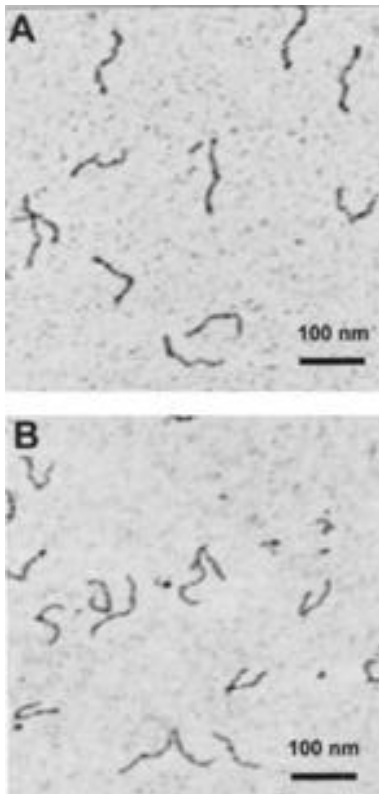
Figure 6. AFM images of sister heteroduplex isomers. These images show different bending angles at the 3-way junctions in the two isomers shown in figure 5 for the 27 bp hairpin (lane 8). (A) Faster migrating isomer. (B) Slower migrating isomer.
