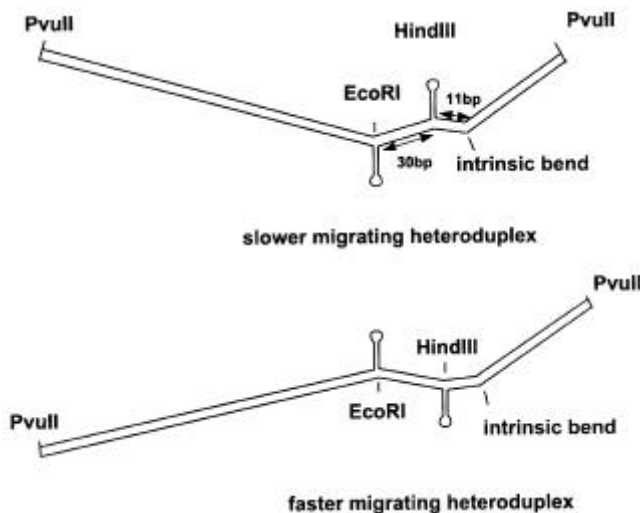
Figure 4. Differential bending in model slipped strand DNA structures. Relationship of hairpin isomer bends to intrinsic bends in DNA is shown. If an intrinsic bend exists in the DNA, then the formation of hairpins (e.g. at the EcoRI and HindIII sites) will introduce a second and third bend in the DNA. The direction of the hairpin-induced bends in the two sister heteroduplex isomers will be either in- or 180° out-of-phase with each other and with the intrinsic bend, and thus may act to introduce curvature in a concerted or antagonistic fashion in the overall molecule. The slow migrating heteroduplex should have the most distant bends oriented in the same direction (top) while the faster migrating heteroduplex should have these bends oriented in the opposite direction (bottom).
