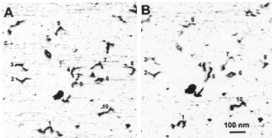
Figure 7. AFM analysis of 3-way junction dynamics in liquid. Two consecutive AFM scans of 301-bp DNA molecules containing a 7-bp hairpin. The DNA, in TE buffer with 200 mM NaCl, was injected into the fluid cell mounted on the top of APS mica. Ten molecules in the field are numbered. Most molecules change shape in the time between the two scans the shape. Molecules 7 and 9, in particular, change shape dramatically. The time between successive scans was 2 min 40 s.
