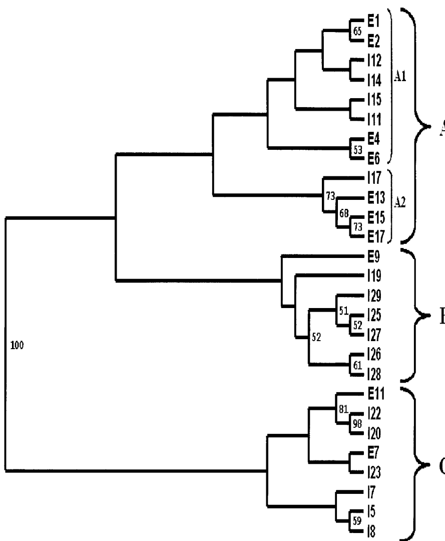
Figure 1. Cluster analysis of SPAR data in case of the mulberry varieties after a 500 replicate bootstrap analysis. The NJ tree was generated for cumulative band data by all three SPAR methods, DAMD, ISSR-PCR and RAPD. The variety names are abbreviated as in table 1, and are indicated to the right of the tree. The branch lengths are based on the distance values computed using NJ method and Jaccard coefficient in the program Free-Tree. The numbers at the nodes in each tree are the bootstrap percent values (only values greater than or equal to 50 are shown) for the branches to the right of the node. The large parenthesis to the right labelled with A-C are the three major clusters while the two inner parenthesis labelled A1 and A2 are the two subclusters within cluster A.
