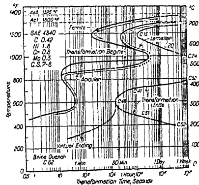
FIG. 2. Isothermal transformation curve for S. A. E. 4340 (Ref. 6).
