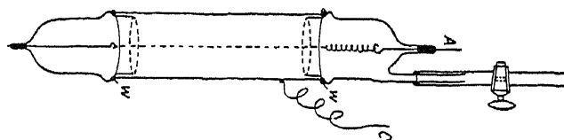
FIG. 2. Thin-walled Geiger-Muller counter A = anode, C = Cathode, W = Wax seal
