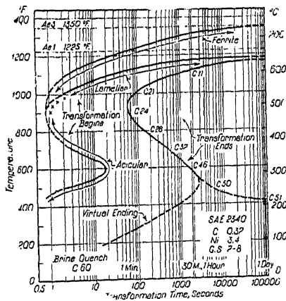
FIG. 1. Isothermal transformation curve for S. A. E. 2340 steel (Ref. 6).
