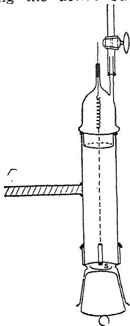
FIG. 7. Soft \beta -ray counter. S = specimen holder.
