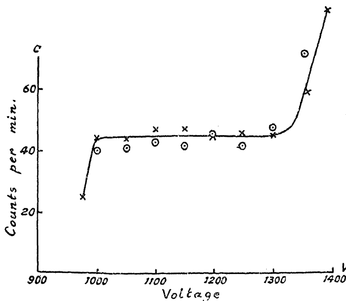
FIG. 9. Characteristic of a demountable soft \beta -ray counter. Circles—when the counter was first assembled. Crosses—after two months of use. drum was such that the absorbers formed a cover for the specimen holder. This prevented
