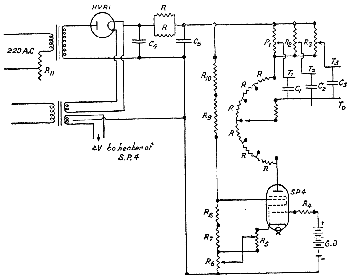
FIG. 4. Stabilised high tension unit for Geiger counters.
