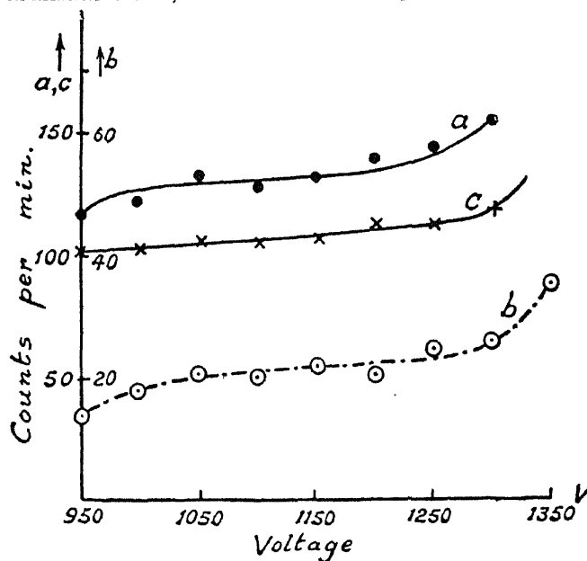
FIG. 6. Characteristic of a Geiger counter
