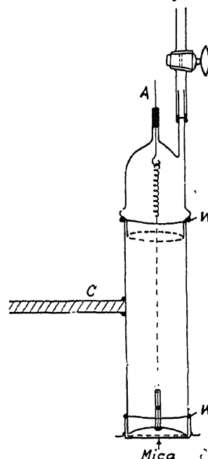
FIG. 3. Grid counter
