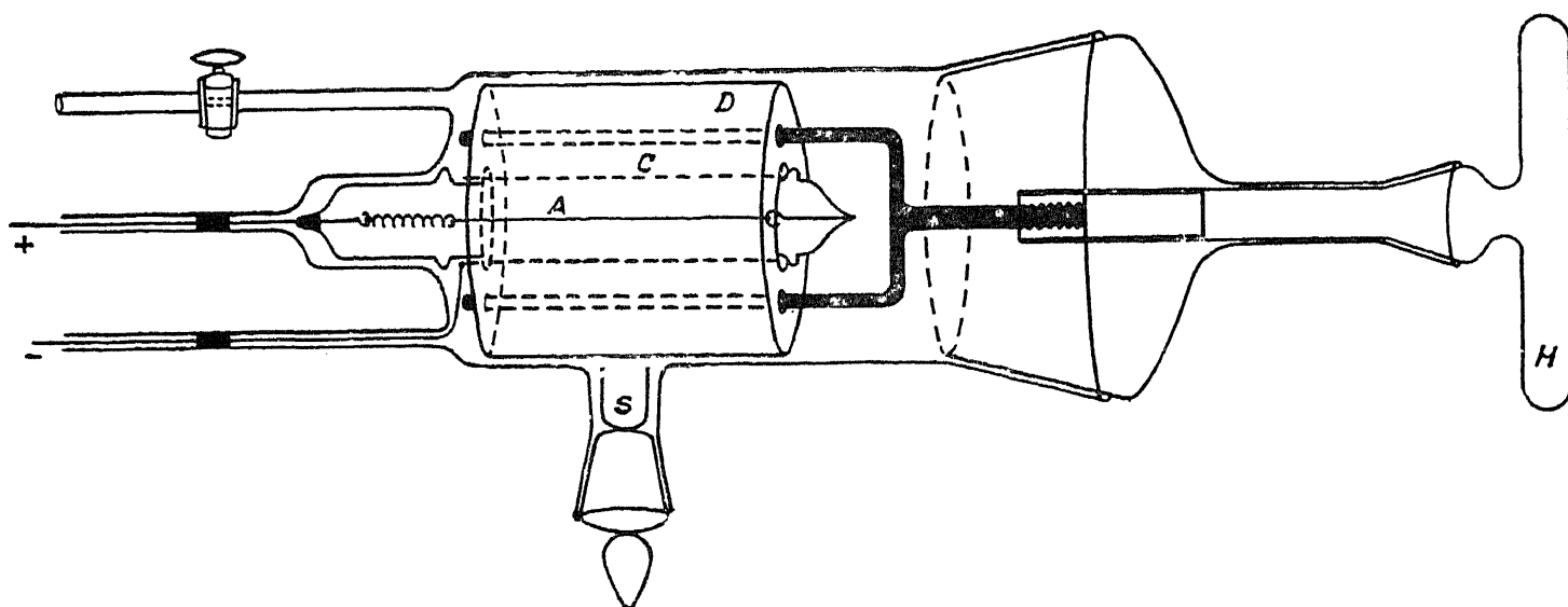
FIG. 8. Demountable soft \beta -ray counter. A = anode, C = cathode; D = drum containing the absorbers; S = specimen holder and H = handle for rotating the drum.
