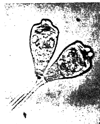
FIG. 3 Two individuals of the colony of Zoothamnium sp. enlarged × 675.
