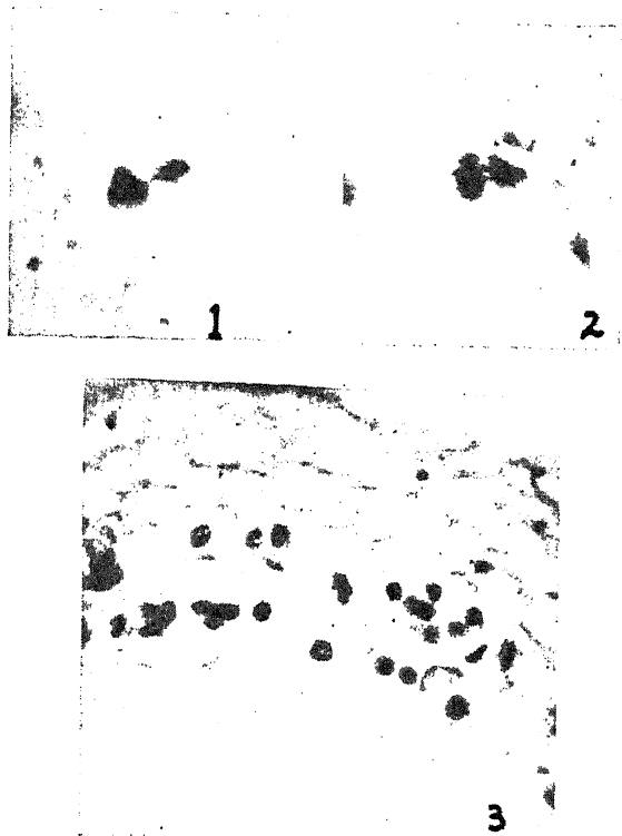
FIGS. 1-2 Extension of chromatin material.
