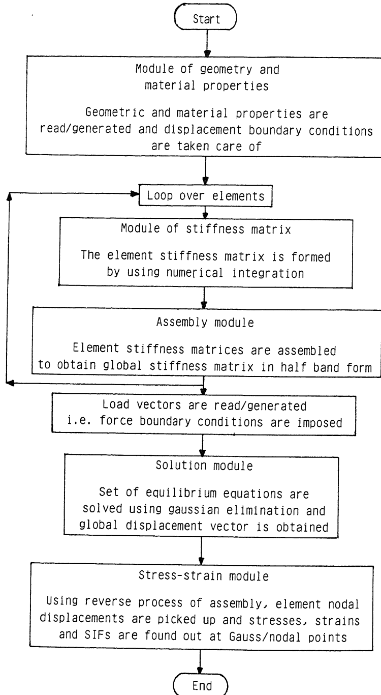
Figure 4. Flow chart used in the FEM oriented computer calculation.
