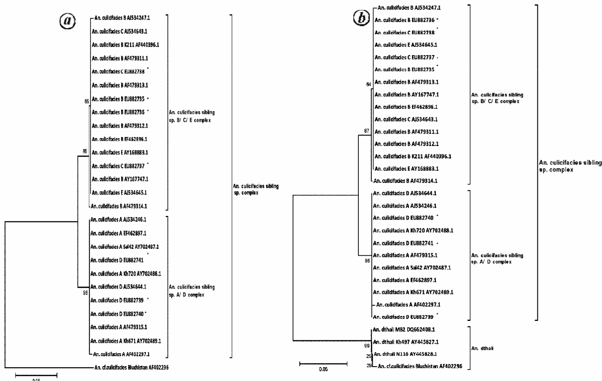
Figure 1. a, Phylogenetic analysis based on rDNA-ITS2 sequences revealed the formation of two separate clades by members of A. culicifacies complex and A. cf. culicifacies 'Bluchistan'. b, The phylogenetic analysis shows the formation of separate clades by A. culicifacies complex and together by A. cf. culicifacies 'Bluchistan' with A. dthali . The accession numbers of new sequences are indicated with asterisk mark (*).
