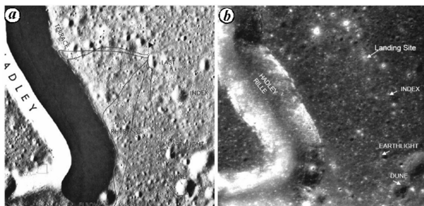
Figure 2. a , Apollo-15 traverses as mapped by NASA on to a high-resolution images acquired during descend of Apollo-15 landing module; b , Corresponding image of Chandrayaan-1 TMC sensor.
