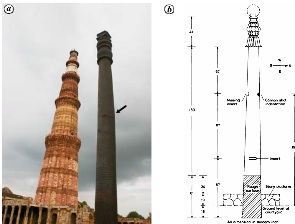
Figure 1. a , Delhi Iron Pillar located at the Quwwat-ul-Islam mosque in the Qutub Complex, New Delhi. Arrow shows the cannon ball strike location on the pillar. b , Salient dimensions of the pillar showing the relative position of the cannon ball indentation and the inserts. The overall symmetric design of the pillar must be appreciated.
