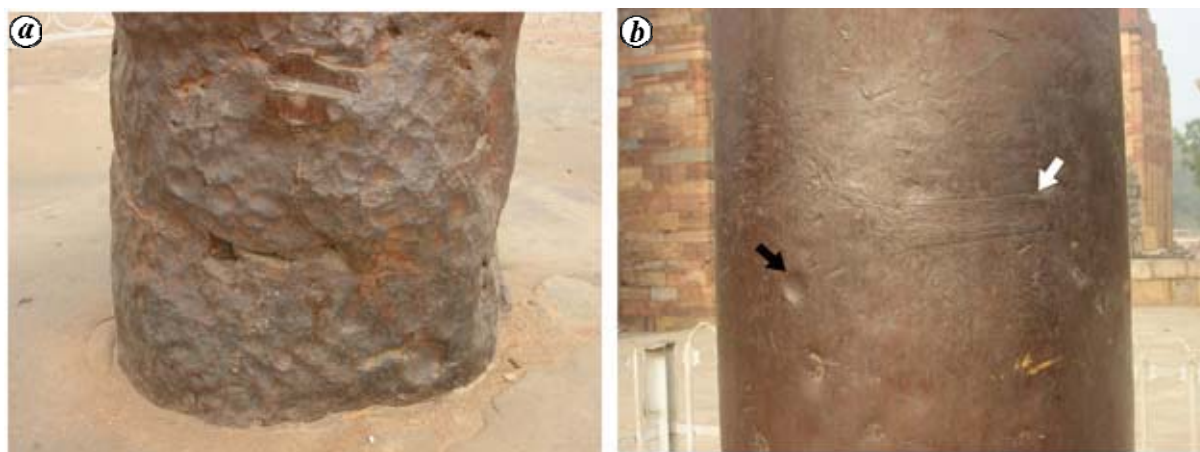
Figure 3. a , Sledgehammer marks on the bottom portion of the pillar due to the original manufacturing technology. b , Indentation mark (black arrow) caused by a shot from the fire arm. The outlines of a rectangular insert can be noted at the location indicated by the white arrow.
