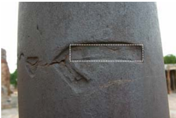
Figure 7. View of the cracked region on the rear, diametrically opposite to the cannon ball strike location. The outline of a previously present horizontal insert is highlighted with dotted line. Note that the material to the left side of the insert was removed by ductile shearing.
