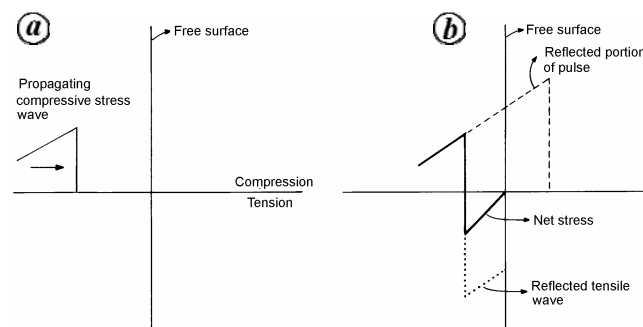
Figure 5. (a) Propagation of compressive stress wave and (b) reflection as a wave from the free surface resulting in net tensile stress near the free surface.
