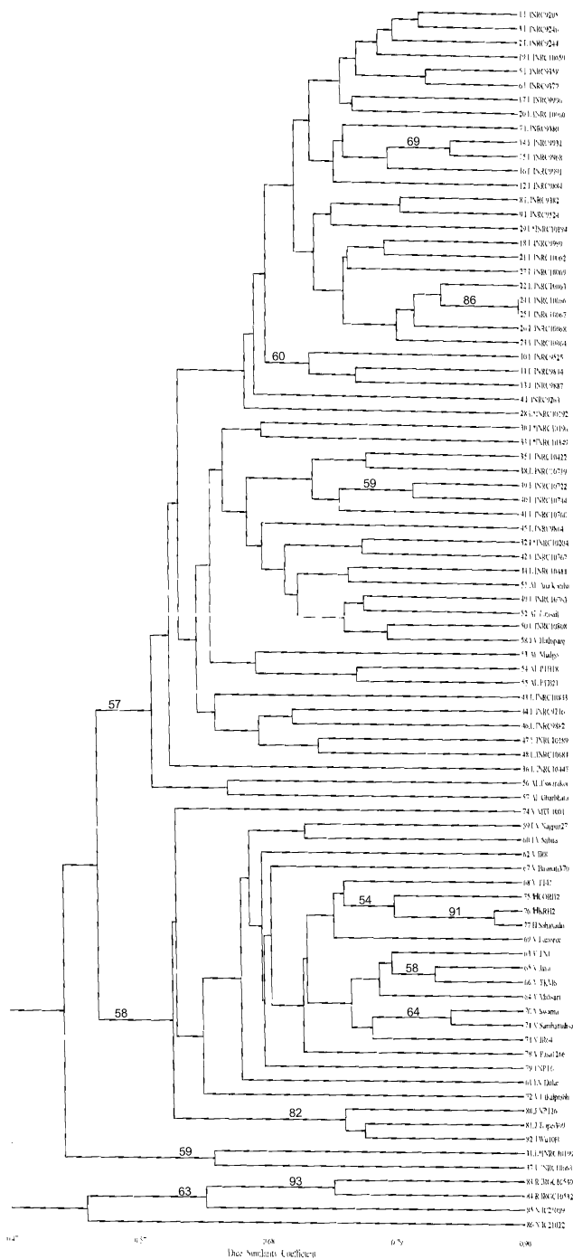
Figure 2. UPGMA dendrogram showing clustering of 86 rice accessions. It is derived from Dice coefficient matrix of 3655 pairwise comparisons using ISSR-PCR data (5514 bands at 220 band positions) from 14 primers. Significant bootstrap values are mentioned on the nodes.
