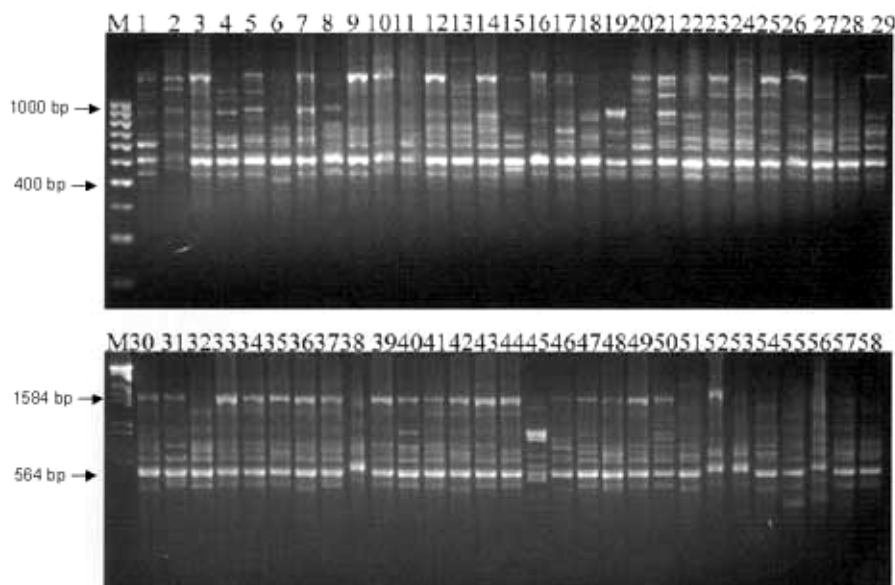
Figure 1. ISSR-PCR amplification profiles of 58 accessions using primer 835. Lanes 1–29 correspond to accessions 1–29 (landraces) respectively, of Table 1 and lanes 30–58 correspond to accessions 58 to 86 (varieties and wild species) respectively, of Table 1. Marker lane at extreme left is 100 base pair DNA ladder (top panel) and lambda DNA/ Eco R1 + Hind III double digest (bottom panel).
