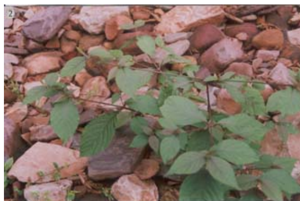
Figure 2. Cyathula prostrata Blume.
