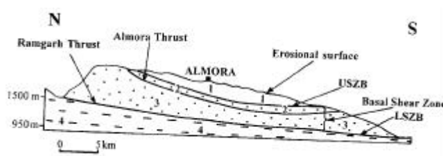
Figure 1. Schematic diagram showing geological setting across the Chhara–Someshwar section of the Almora Nappe. 1, Almora Group; 2, Almora Group mylonites; 3, Ramgarh Group mylonites; 4, Autochthonous sedimentaries of the Damtha and Jaunsar groups; USZB, Upper Shear Zone Boundary; LSZB, Lower Shear Zone Boundary.
