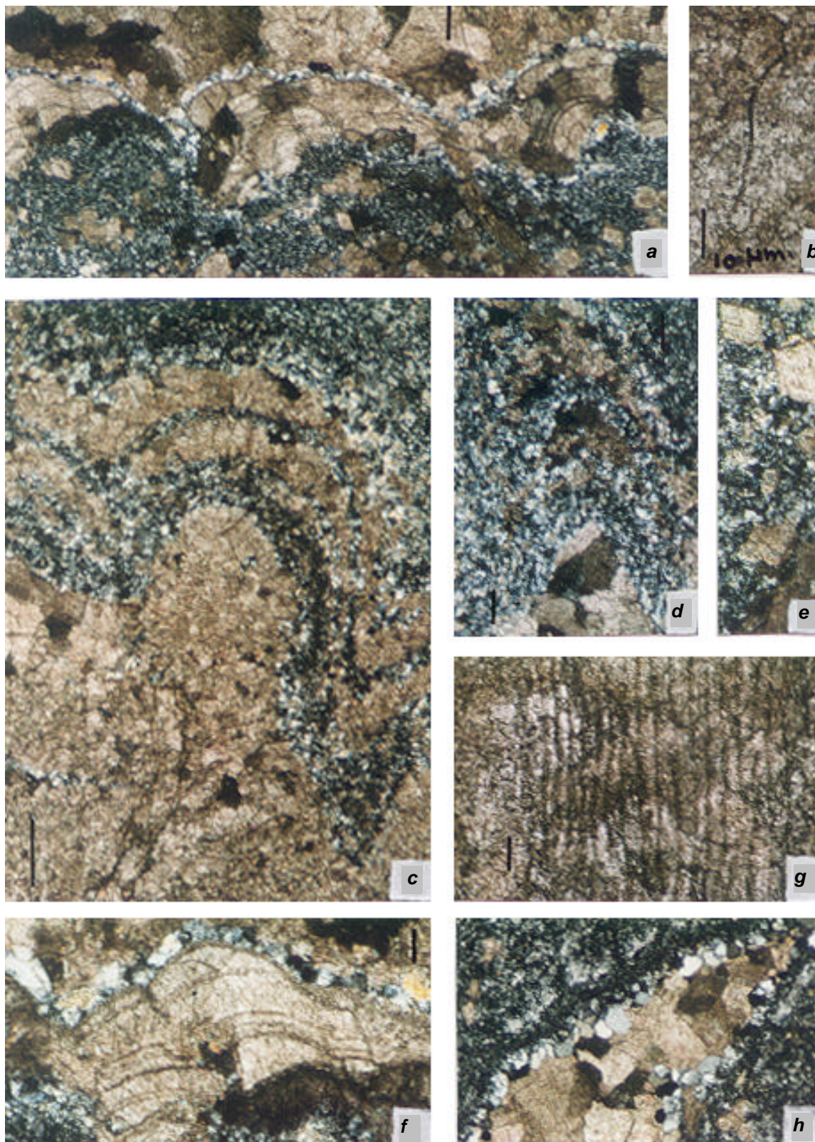
Figure 3. a , Plane polarized light photomicrographs of microstromatolitic build-up of columnar linked-type, microfacies MF3 showing dolomitic microlamina, microsparitic microlamina and sparitic lamina; b , Eomycetopsis , cyanobacterial filamentous microbiota; c , Diagenetic replacement features of MF2 microfacies showing alternate fine chert and quartz layers. A cyclicity has been observed in diagenetic replacement of carbonate microstromatolites by chert/quartz (slide no. MM6a, b), scale bar = 1 mm; d , Recrystallized (sparitic lamina) conical-columnar type microfacies MF2; e , Unzoned and zoned dolorhombs (slide nos. MM1, MM2, MM6b), scale bar = 1 mm; f , Enlargement of columnar linked microstromatolites showing sparitic lamina (top) and micritic microlamina (below) (slide no. MM6a), scale bar = 1 mm; g , Alternate dark and light carbonate layers (Zebra fabric); h , Stromatactis microfacies of the Menga Limestone (slide no. MM6a).
