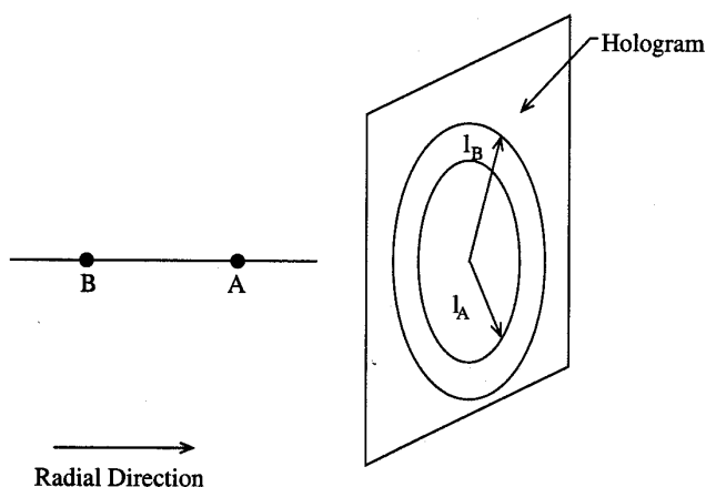
Figure 4. The image of pt A is spreadout over radius I_A . The image of pt B is spreadout over a bigger radius I_B .
