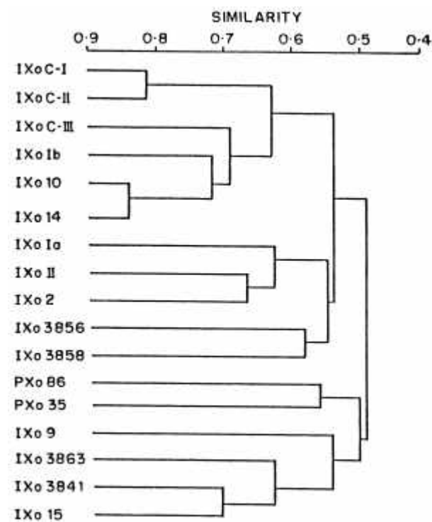
Figure 3. Dendrogram of 15 Indian strains based on similarity index ( X_p ) of Xoo by bacterial identification assays conducted in which probes ( TG ) 10 , pV47, avrXa10 , and pBS101 (ref. 26).
