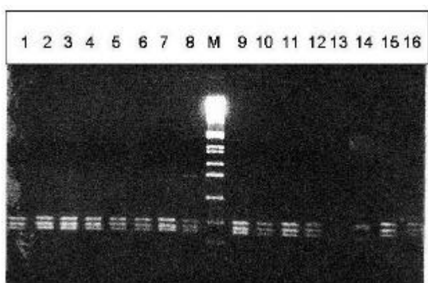
Figure 1. Amplified 16S rDNA of Salmonella enterica strains digested with RsaI .
